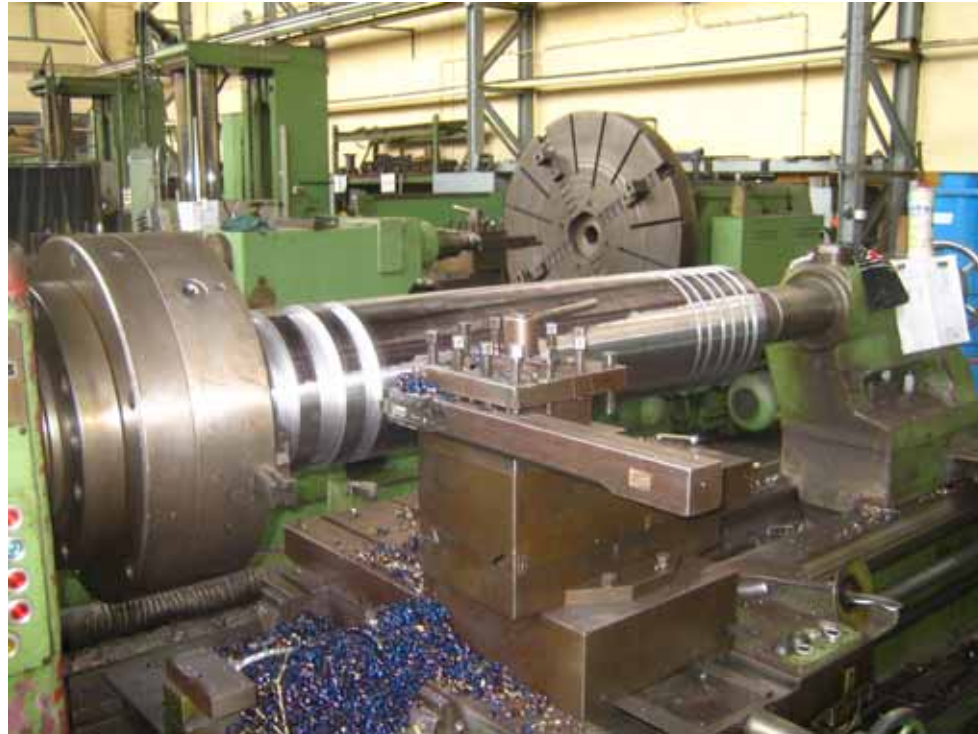
Grooving of the Infeed roll
